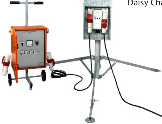
Distribution Trolley & Daisy Chain.
